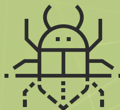
Antivirus software
